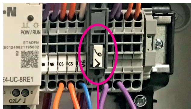
FUSIBLE 5X20 1A ELECTROVANNE AIR
